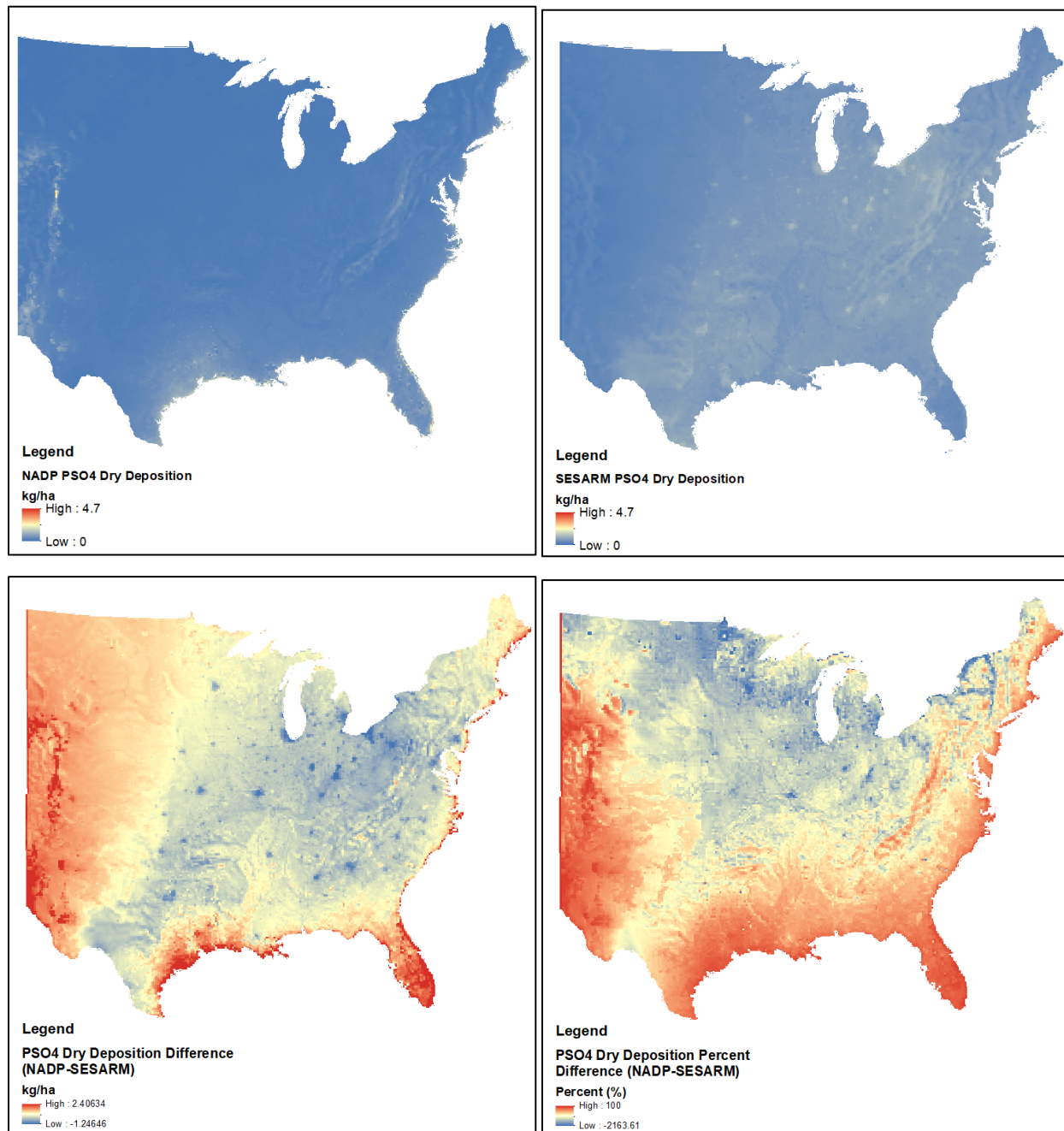
Figure 7-42. Plots of Total Annual Particulate \text{SO}_4^{2-} Deposition. NADP Dry Deposition (top left), SESARM Dry Deposition (top right), Difference (bottom left), Percent Difference 104 (bottom right).
