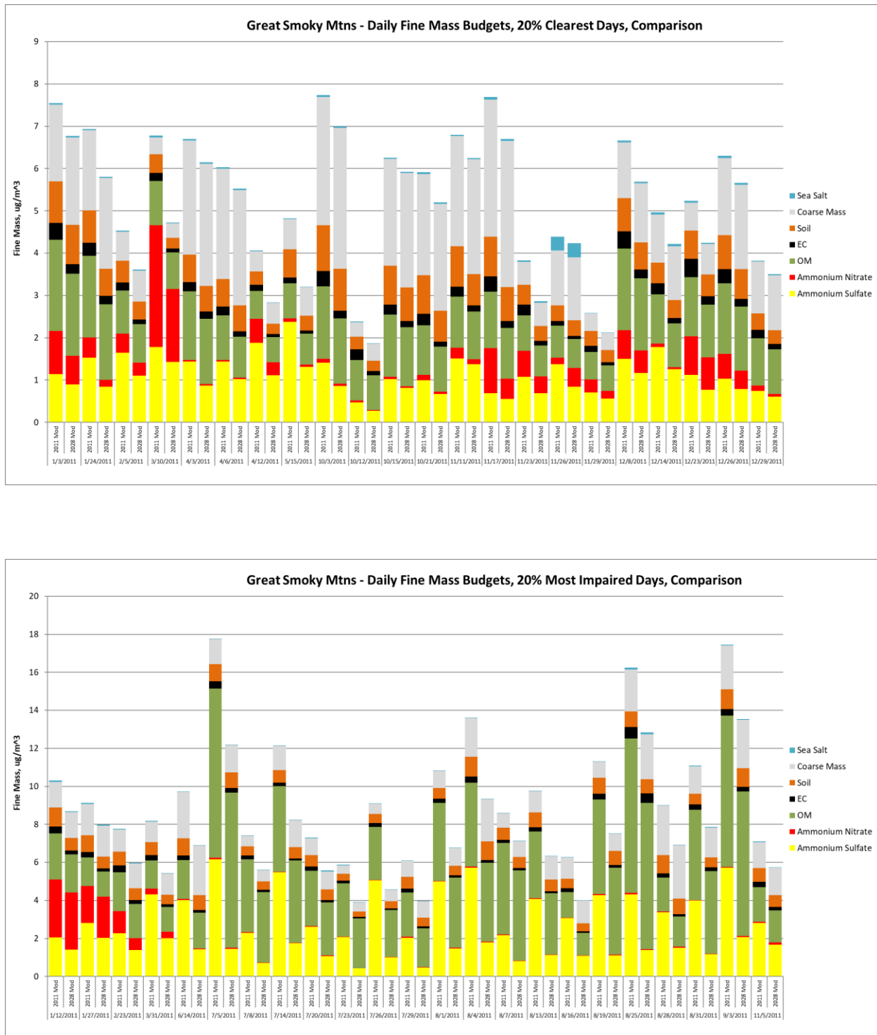
Figure 10-4. Predicted (CAMx) Concentrations ( \mu\text{g}/\text{m}^3 ) Great Smoky Mountains National Park on the Modeled 20% Clearest (Top) and 20% Most Anthropogenically Impaired (Bottom) Days.
