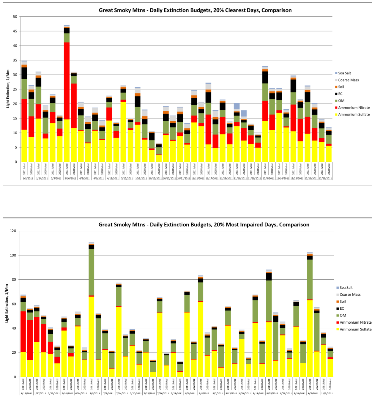
Figure 10-5. Predicted (CAMx) Light Extinctions ( \text{Mm}^{-1} ) Great Smoky Mountains National Park on the Modeled 20% Clearest (Top) and 20% Most Anthropogenically Impaired (Bottom) Days.
